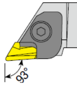
CKJNR/L (Top Clamp Type 93°)
