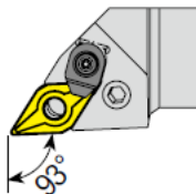
PDJNR/L (Lever Type 93°)
